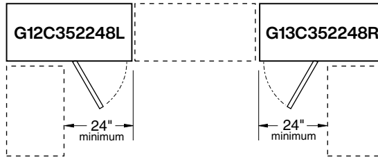
PLAN VIEW OF G12C352248L & G13C352248R
